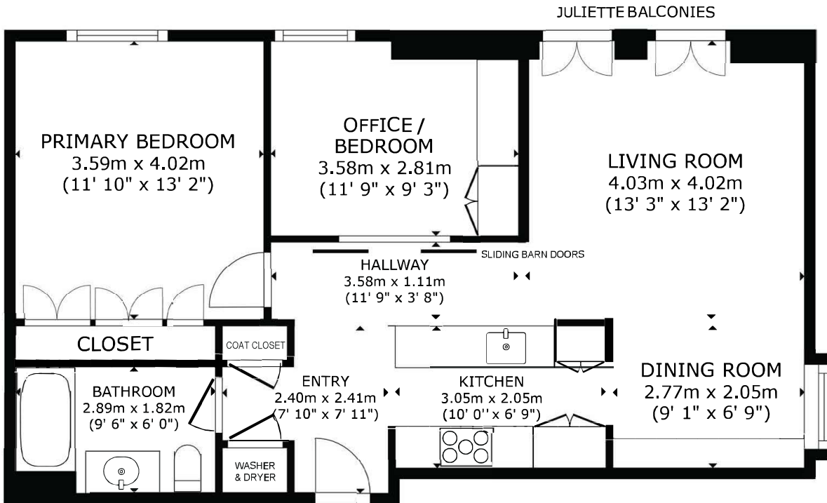
FLOOR PLAN
